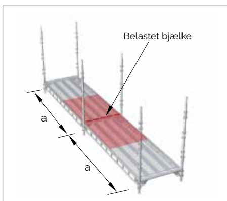
Facadestillads
